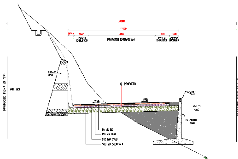
TCS-IV Two Lane With Paved Shoulder (One Side Hill One Side Valley Section) (No Alignment)
