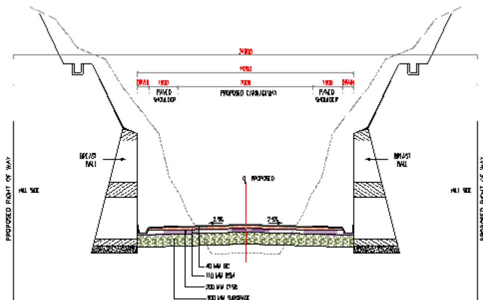
TCS-VII Two Lane With Paved Shoulder Concentric Widening (Both Side Hill Section)
