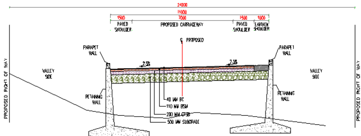
TCS-VIII Two Lane With Paved Shoulder (Both Side Valley Section) (R&A Alignment)
