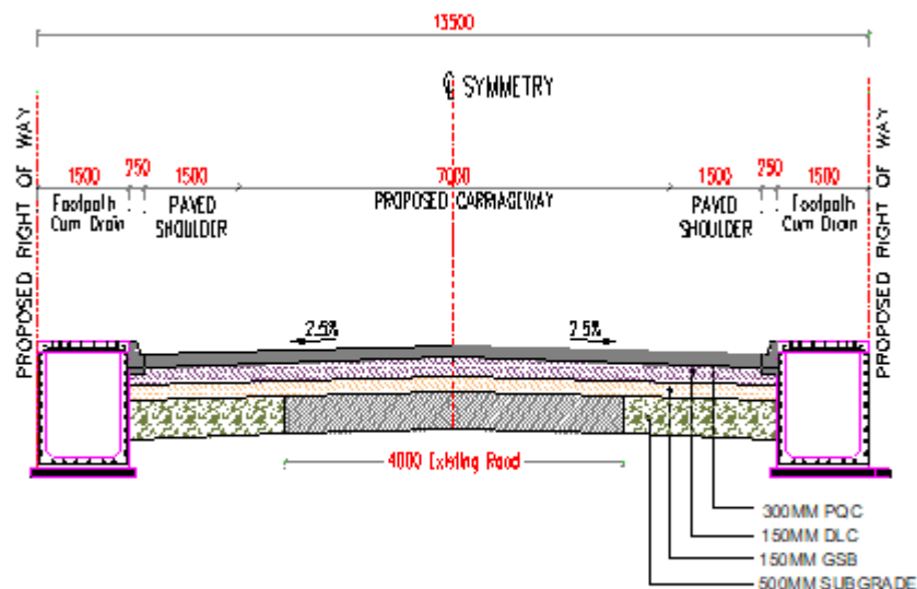
TCS-X Two Lane Carriageway With Paved Shoulders Including Both Side Drain Cum Footpath (Building Area-Mountainous Terrain)
