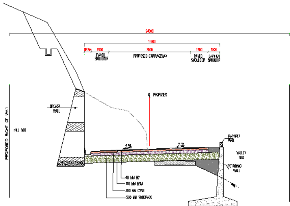
TCS-II Two Lane With Paved Shoulder Eccentric Left Side Widening (One Side Hill One Side Valley Section)
