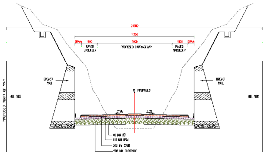
TCS-V Two Lane With Paved Shoulder (Concentric Widening (Both Side Hill Section))
