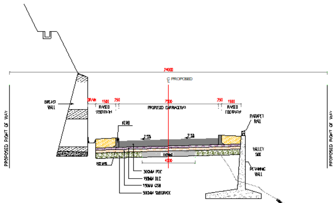
Typical Cross-Section - IX Two Lane Carriageway With Raised Footpath Parking Area (R&A Alignment)
