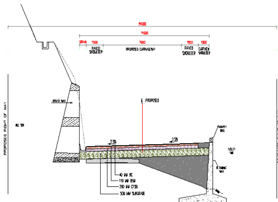
TCS-III Two Lane With Paved Shoulder Eccentric Right Side Widening (One Side Hill One Side Valley Section)
